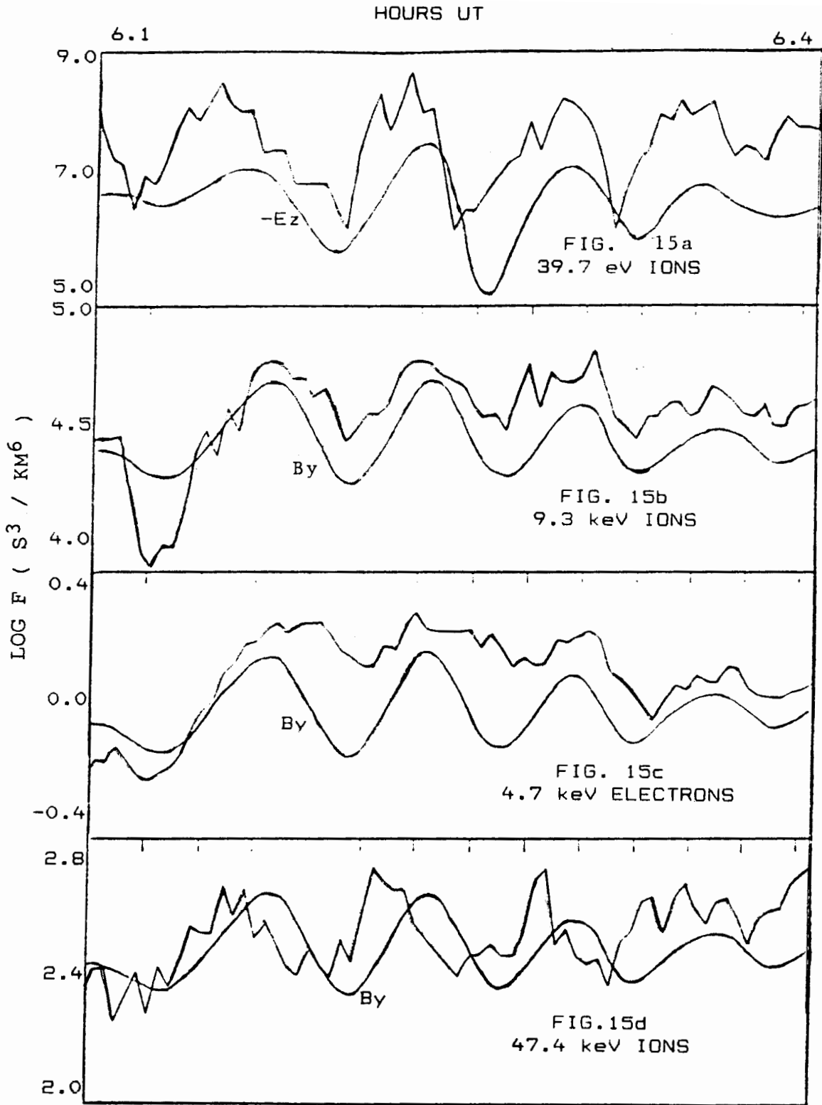
Figure 15. Ion and Electron Distribution Functions
